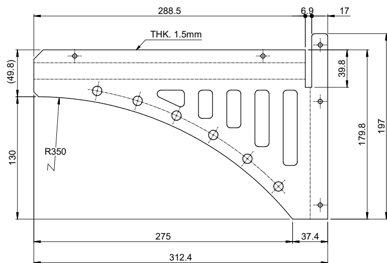
DEVELOPMENT SHEET METAL
