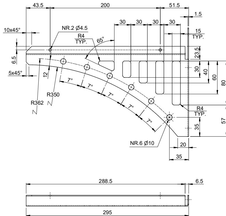
DEVELOPMENT SHEET METAL
