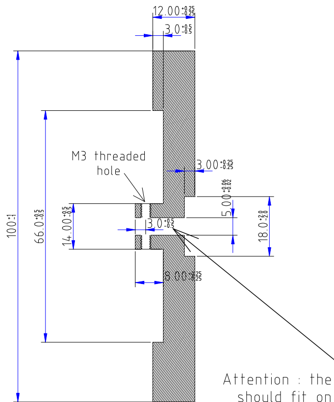
Cutting view
