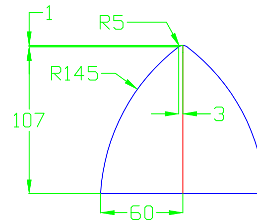
Profile B
