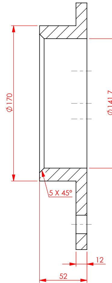
SECTION C-C
