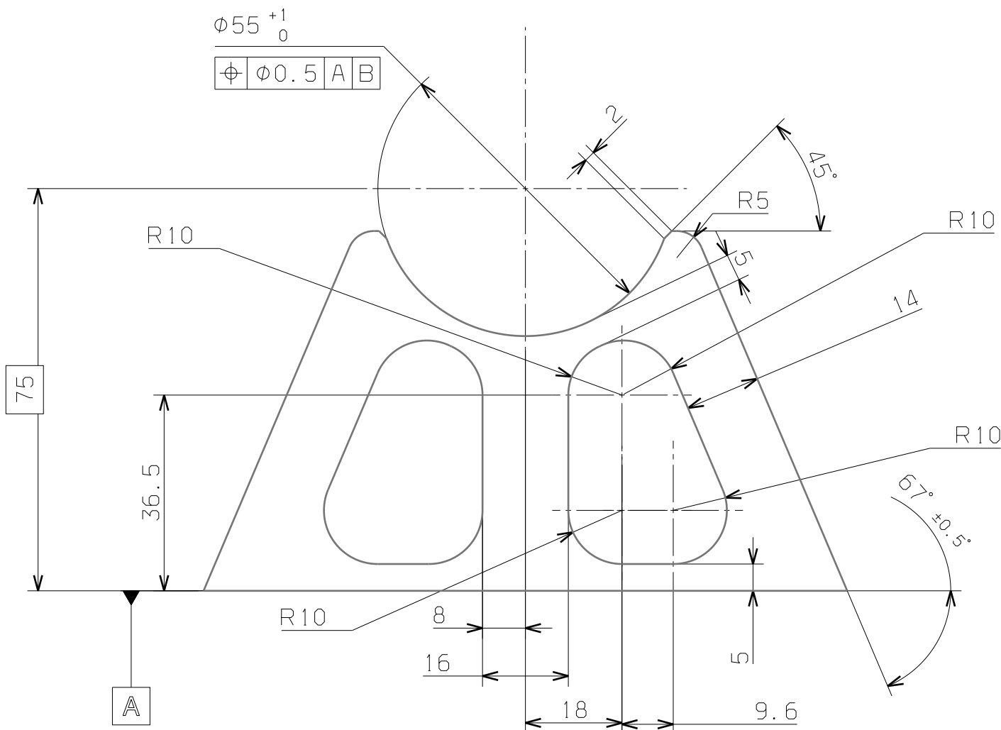
Front view
