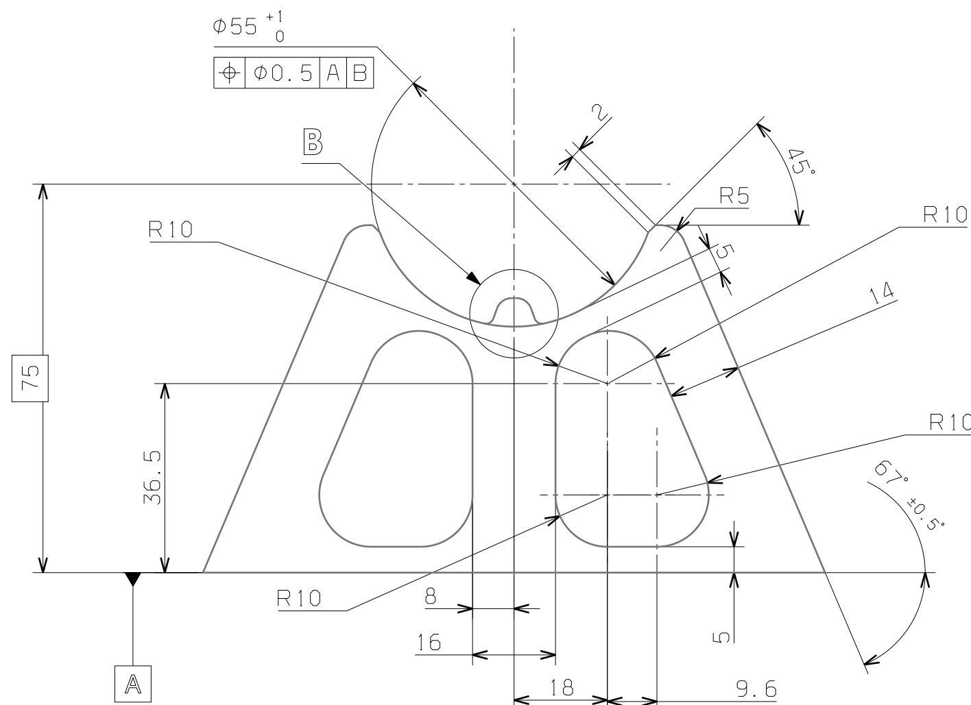
Front view
