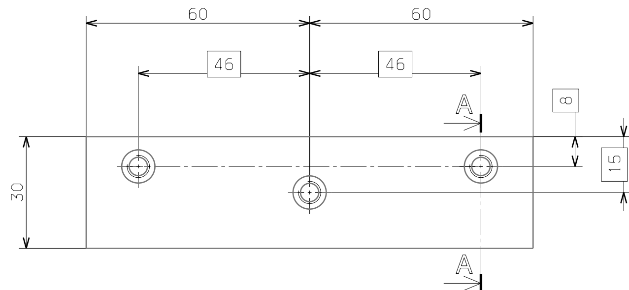
Bottom view
