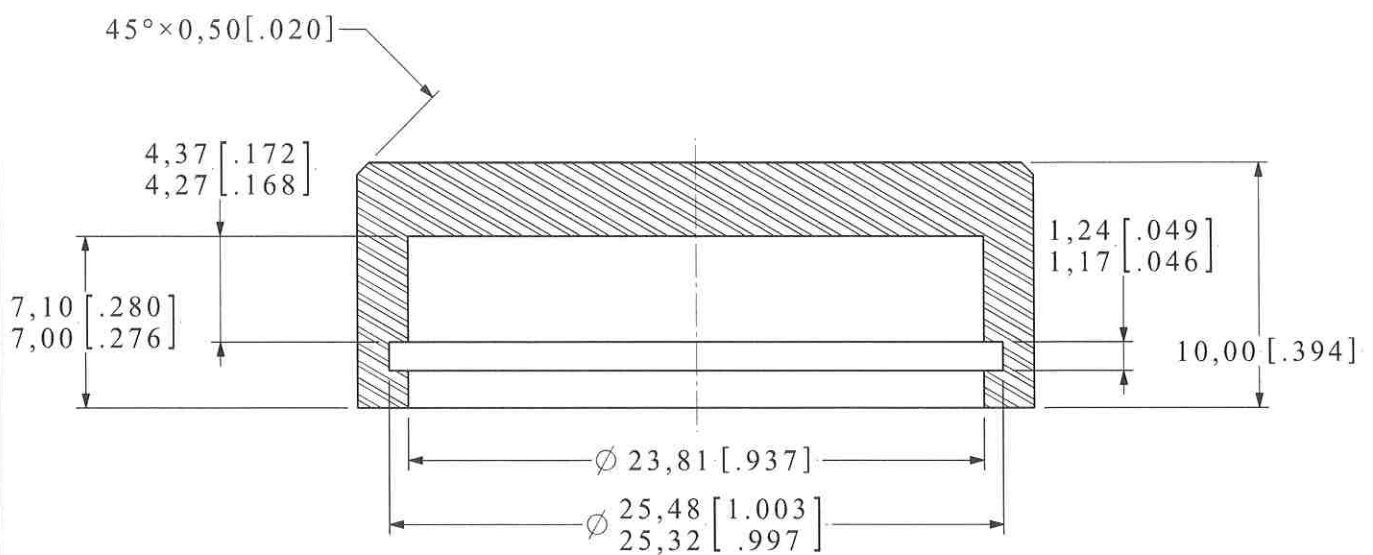
SECTION BB-BB (H4)
