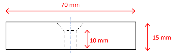
3 – side view
