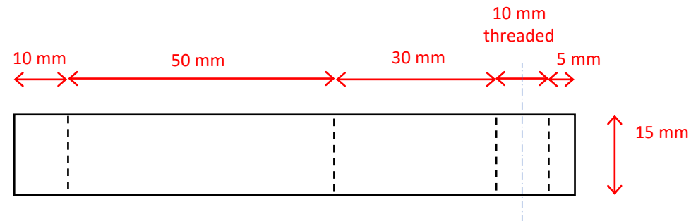
3 – front view
