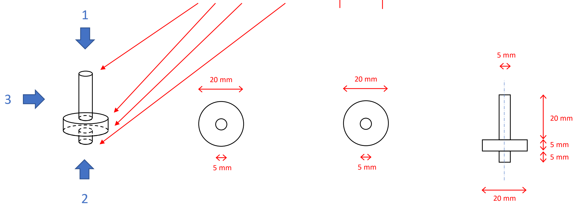
perspective view
