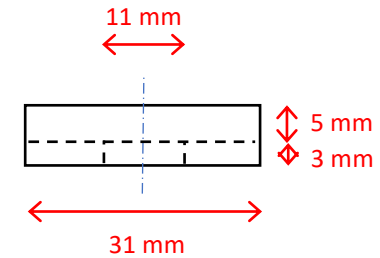
4 – side view
