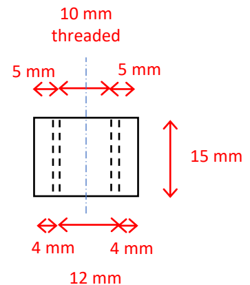
4 – side view
