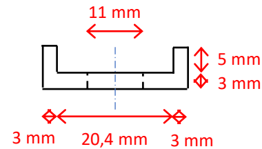
3 – front view
