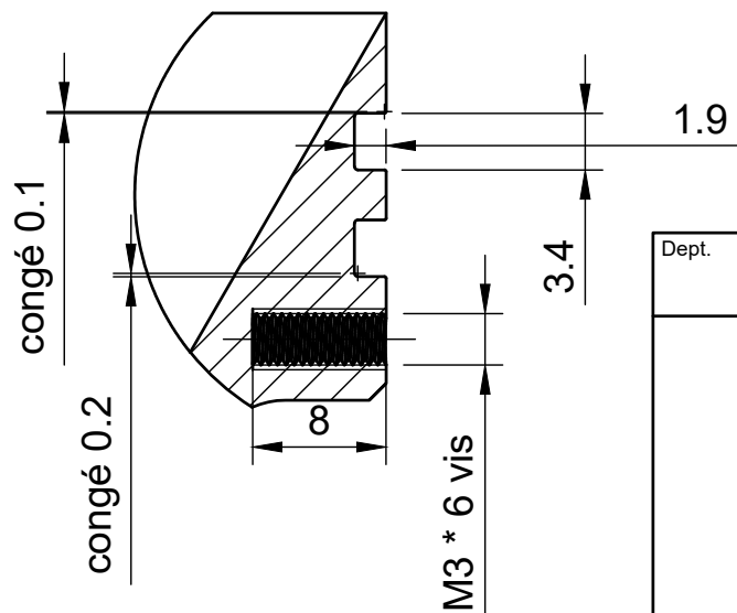
B (2:1) Joint Torique & vis
