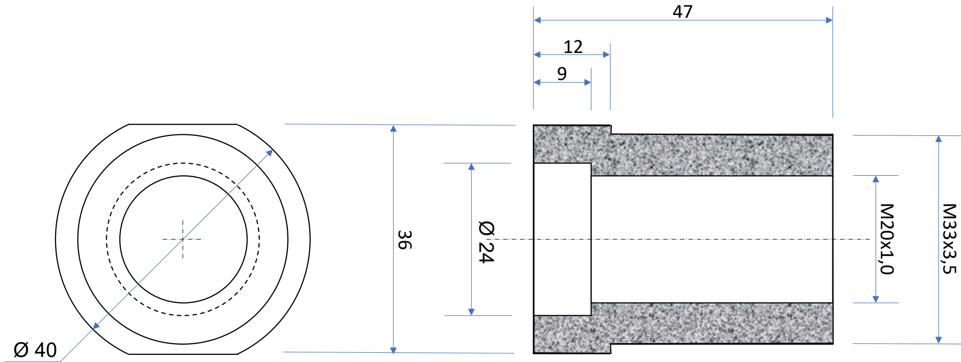
Bague adaptation tour M20x1,0 – M33x3,5 Matière: Acier C35
