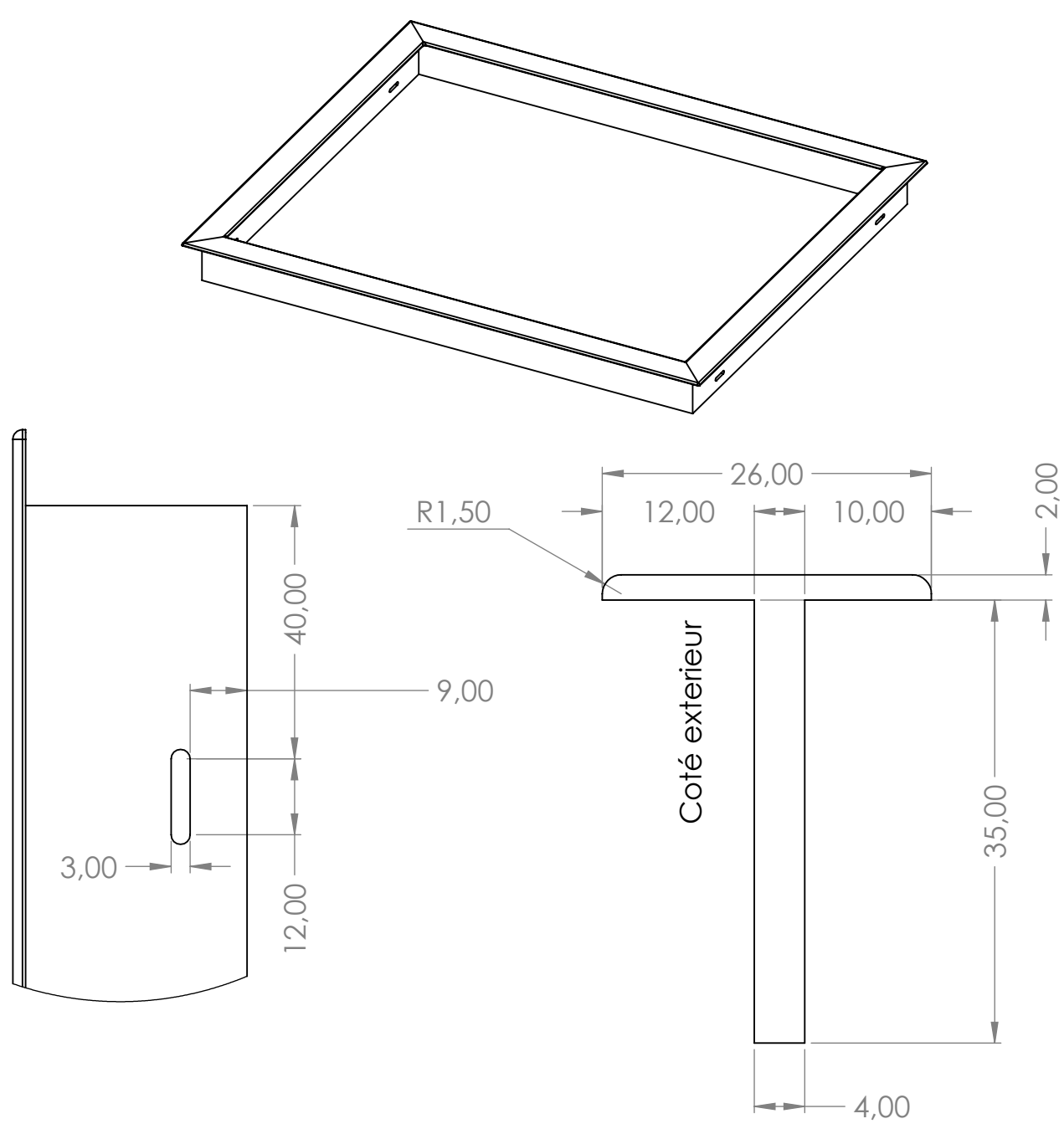
DETAIL A SCALE 1 : 1
