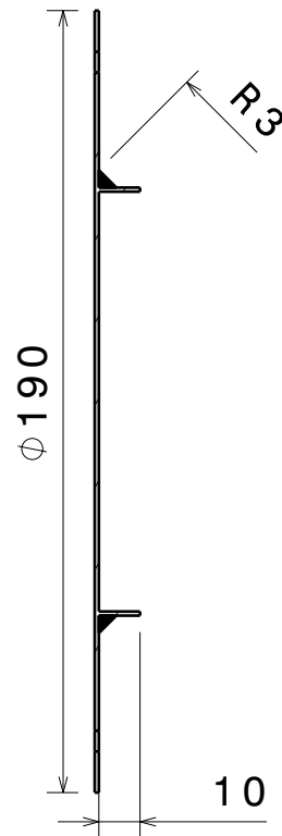
Section view H-H Scale: 1:2
