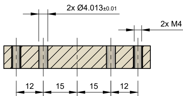
B-B (1:1)
