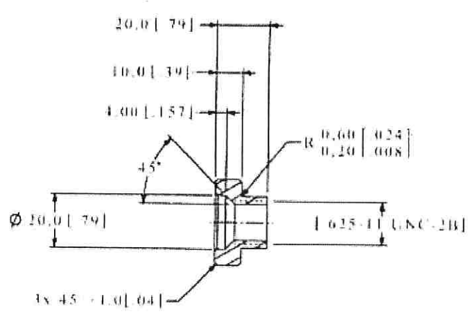
SECTION W-W (113)
