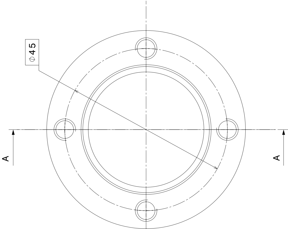
Front view Scale: 2:1
