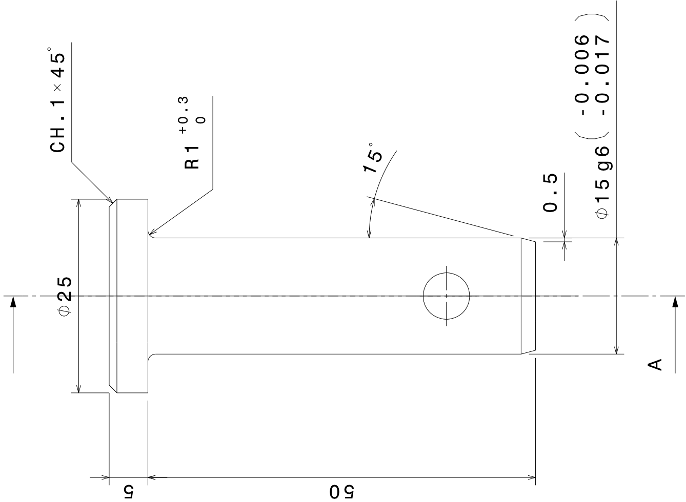
Front view A Scale: 2:1
