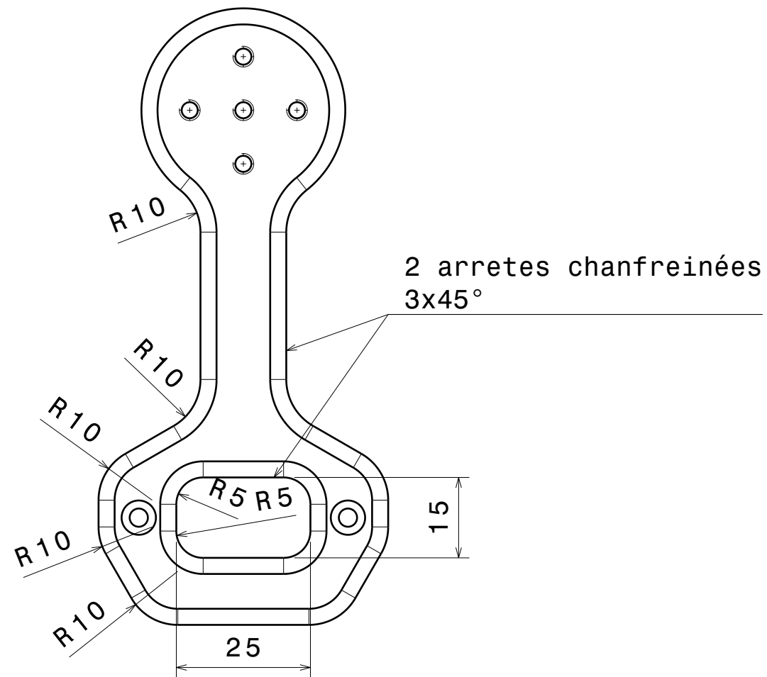
Back view Scale : 1:1
