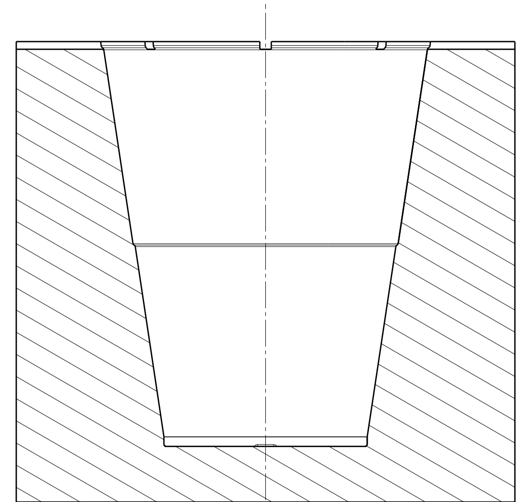
Section view F-F Scale: 1:1
