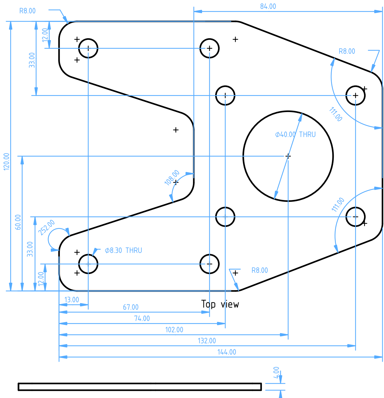
Front view
