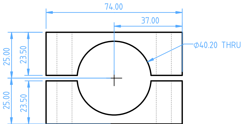
Front view
