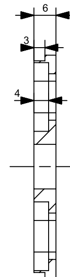
SECTION B-B
