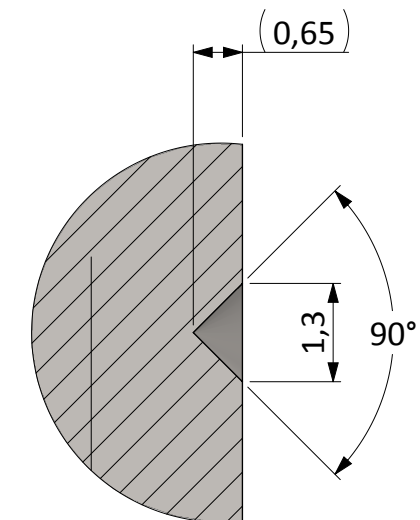
DETAIL B SCALE 10 : 1
