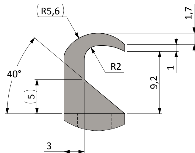
DETAIL C SCALE 3 : 1
